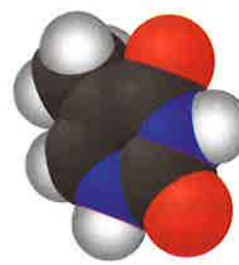
Thymine
