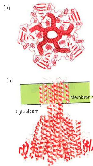
Figure 8 Magnesium channel
