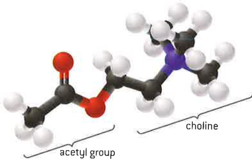
▲ Figure 16 Acetylcholine
