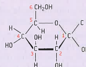
▲ Glucose
