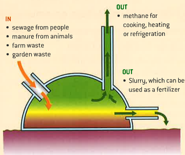
▲ Figure 7 Methane generator. Conditions inside must be anaerobic
